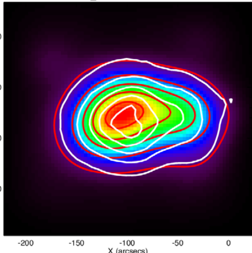
GX 5.7 GHz T_I 12-Jul-2012 04:58:25.900 UT
