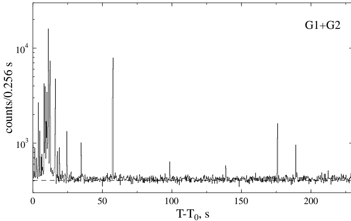
Fig. 3.6.— General pattern of the event 980530a. The first series of numerous soft bursts.
