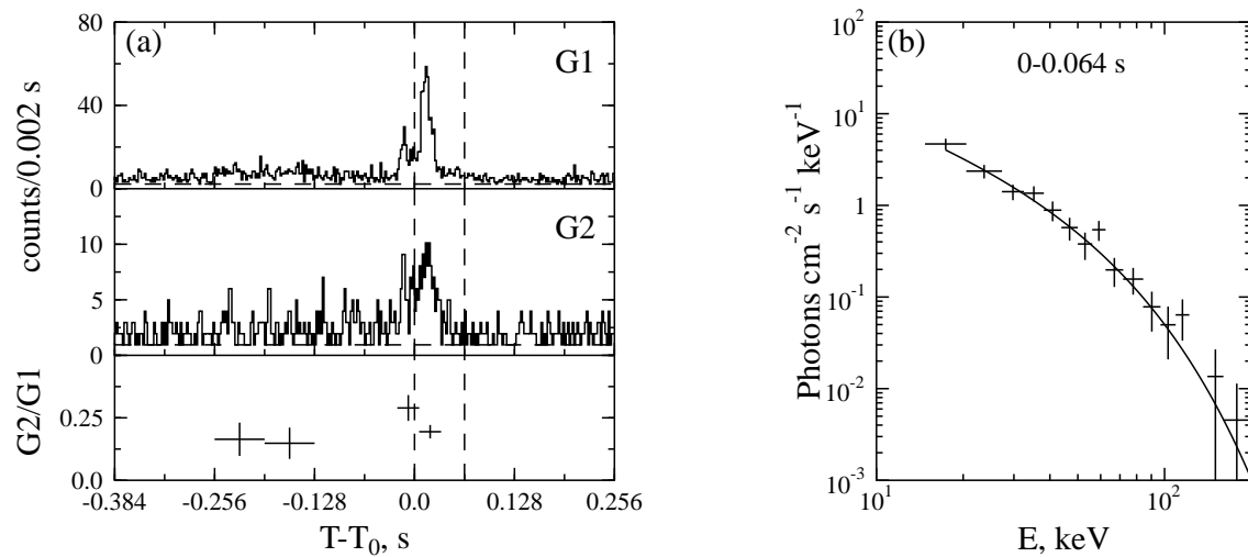
Fig. 3.7.— Starting burst in the event 980530a. (a) – time structure. (b) – energy spectrum.
