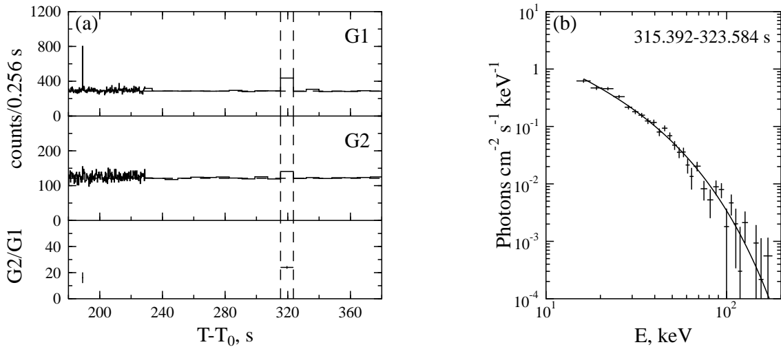
Fig. 3.15.— Event 980530a (continued). See comments to Fig. 3.42.
