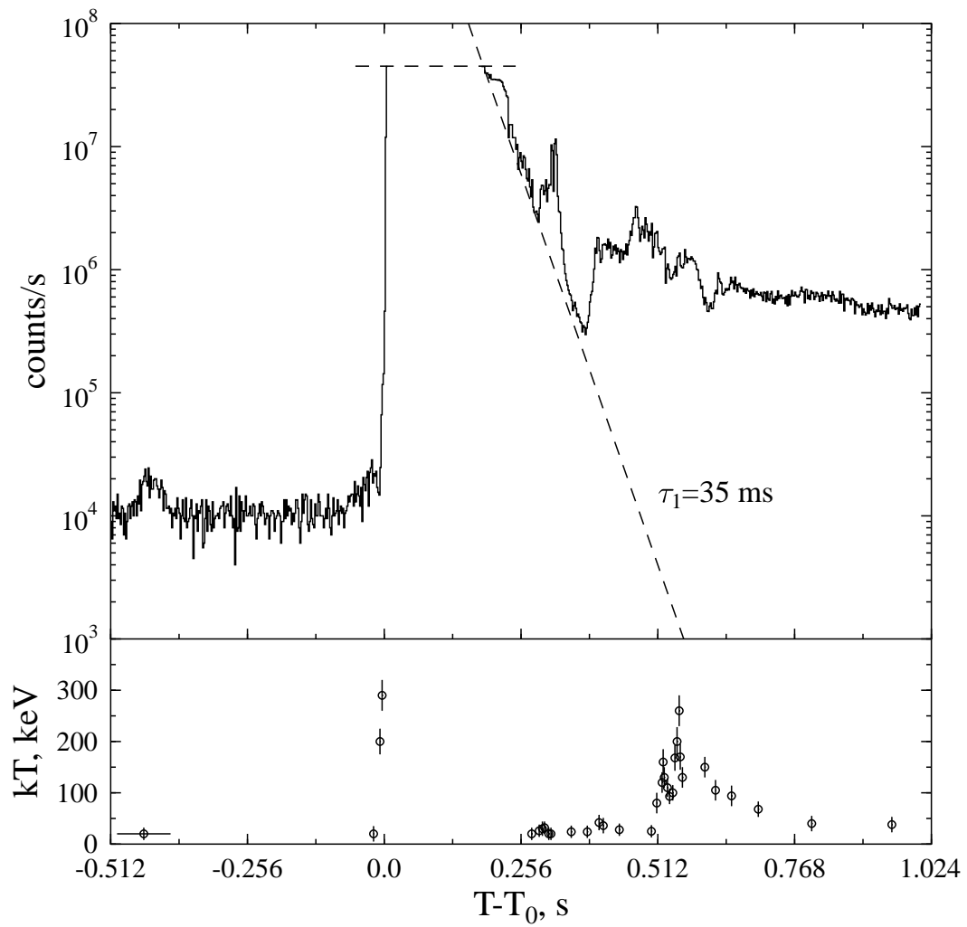
Fig. 3.28.— Initial pulse of the outburst 980827.
