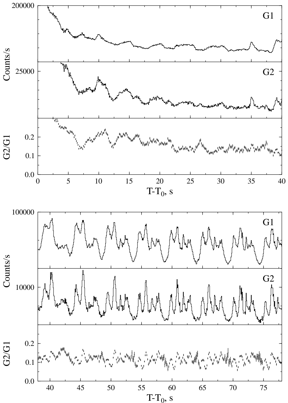
Fig. 3.29.— Pulsating tail of the 980827 outburst.
