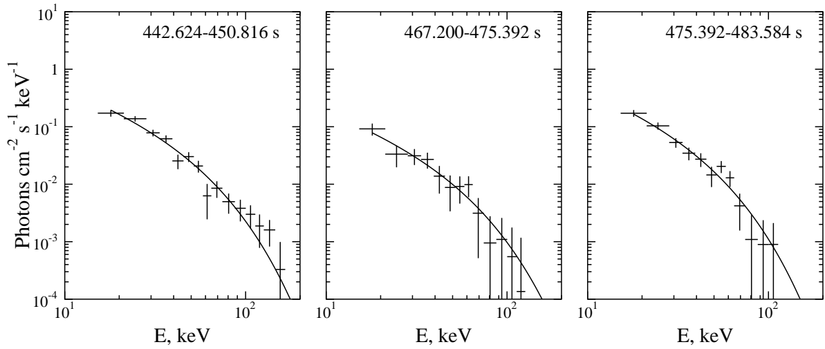
Fig. 3.58.— Event 981024. Energy spectra of the final phase (continued).
