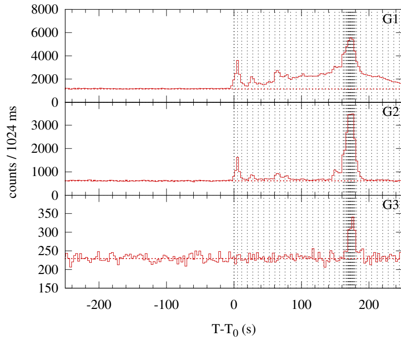
Konus-WIND S1 SOL1995-02-03T01:47 (M4.3) T_0 = 6431.728 s UT (01:47:11.728)
