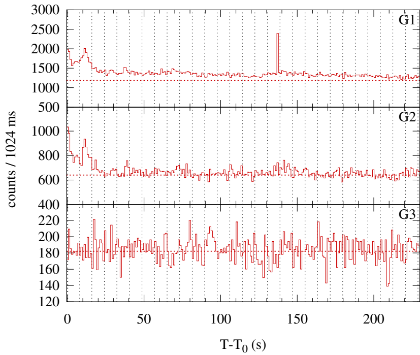
Konus-WIND S2 SOL1995-02-20T03:18 (M1.1) T 0 = 11907.878 s UT (03:18:27.878)
