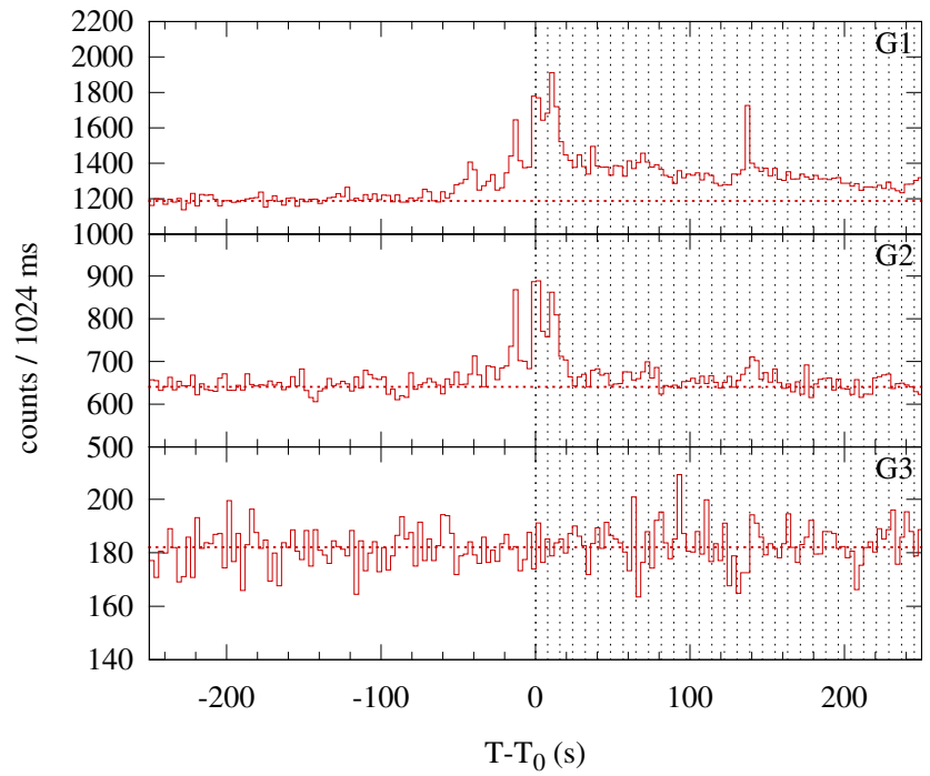
Konus-WIND S2 SOL1995-02-20T03:18 (M1.1) T 0 = 11907.878 s UT (03:18:27.878)
