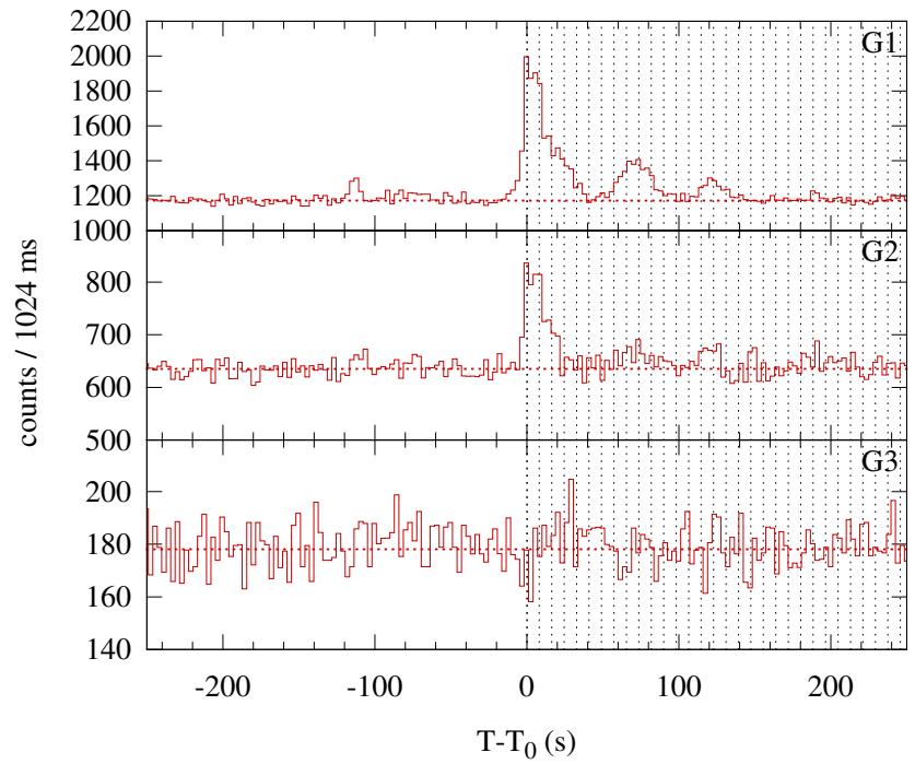
Konus-WIND S2 SOL1995-03-29T06:47 (C1.6) T_0 = 24465.958 s UT (06:47:45.958)
