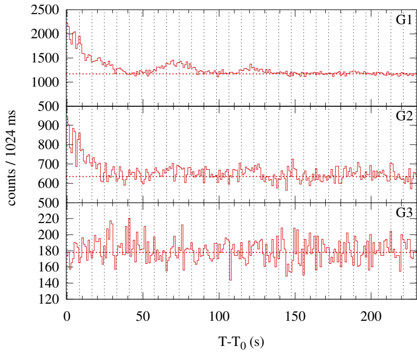
Konus-WIND S2 SOL1995-03-29T06:47 (C1.6) T_0 = 24465.958 s UT (06:47:45.958)
