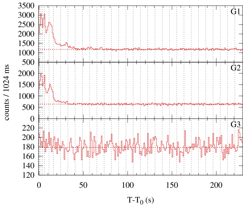
Konus-WIND S2 SOL1995-03-29T18:51 (C1.9) T_0 = 67912.697 s UT (18:51:52.697)
