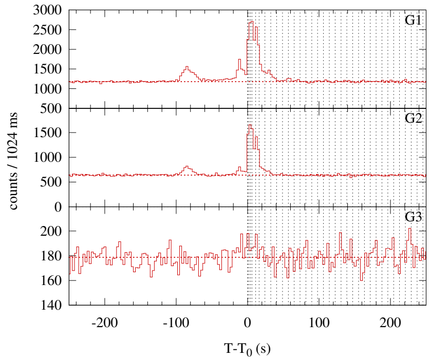
Konus-WIND S2 SOL1995-03-29T18:51 (C1.9) T_0 = 67912.697 s UT (18:51:52.697)
