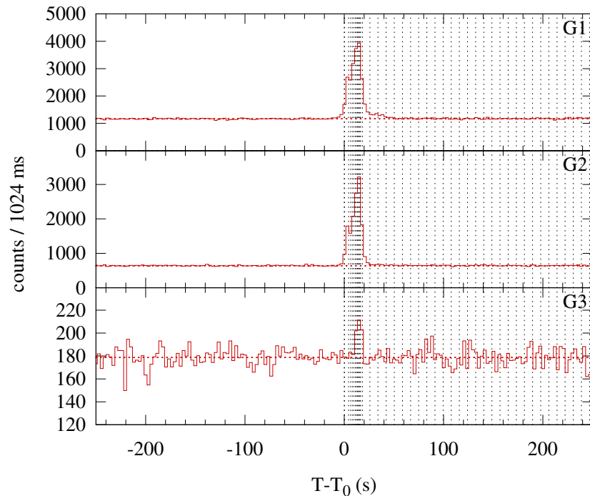
Konus-WIND S2 SOL1995-03-29T21:56 (B6.6) T_0 = 78970.723 s UT (21:56:10.723)
