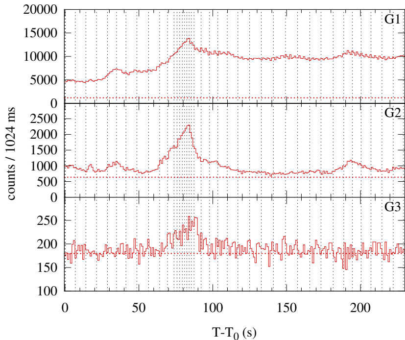
Konus-WIND S2 SOL1995-04-22T11:45 (M7.1) T_0 = 42322.690 s UT (11:45:22.690)
