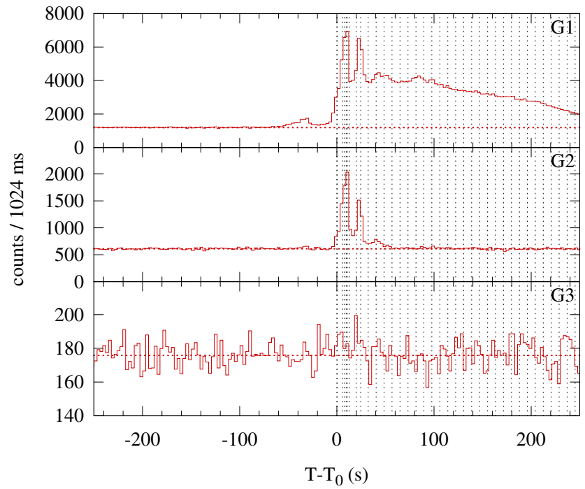
Konus-WIND S2 SOL1995-10-13T05:01 (M4.8) T_0 = 18117.517 s UT (05:01:57.517)
