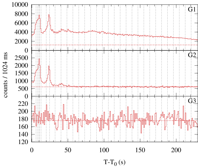
Konus-WIND S2 SOL1995-10-13T05:01 (M4.8) T_0 = 18117.517 s UT (05:01:57.517)
