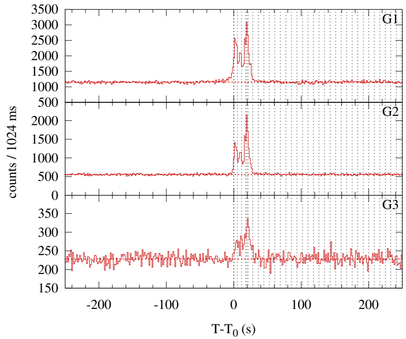
Konus-WIND S1 SOL1997-09-22T00:48 (C1.7) T_0 = 2889.663 s UT (00:48:09.663)
