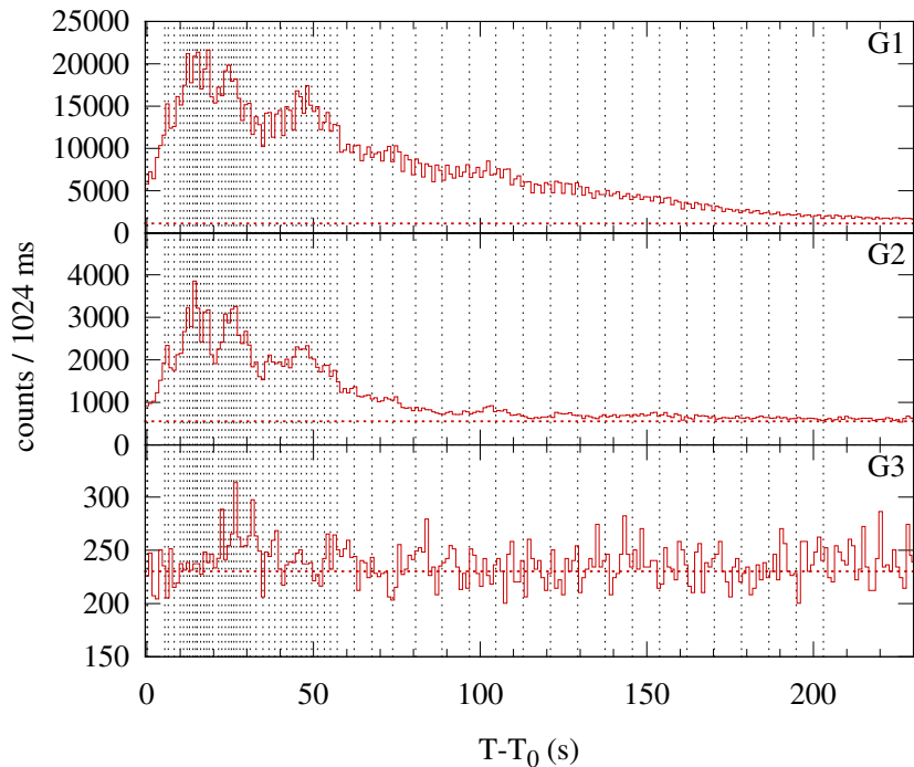
Konus-WIND S1 SOL1997-09-24T02:46 (M5.9) T 0 = 10001.465 s UT (02:46:41.465)
