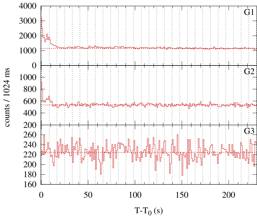
Konus-WIND S1 SOL1997-11-27T13:03 (X2.6) T 0 = 47026.785 s UT (13:03:46.785)
