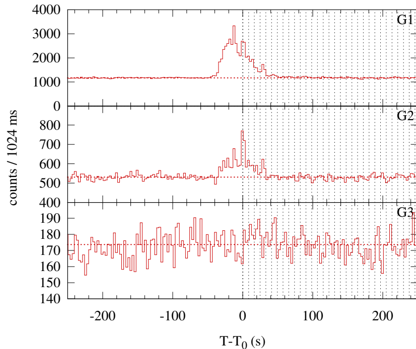
Konus-WIND S2 SOL1998-03-05T23:08 (C5.6) T_0 = 83296.27 s UT (23:08:16.27)
