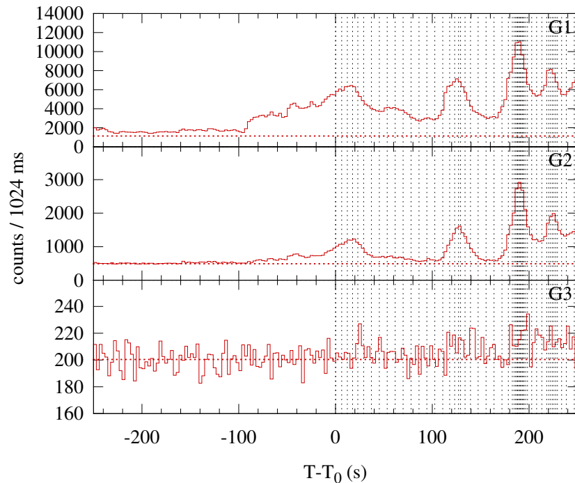
Konus-WIND S1 SOL1998-09-23T06:52 (M7.1) T_0 = 24721.914 s UT (06:52:01.914)
