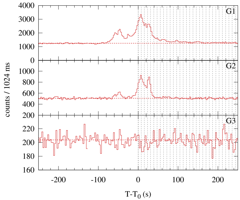
Konus-WIND S1 SOL1998-09-28T12:00 (C9.5) T 0 = 43216.505 s UT (12:00:16.505)
