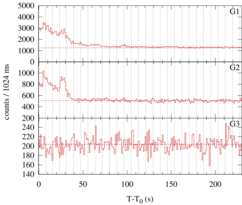
Konus-WIND S1 SOL1998-09-28T12:00 (C9.5) T 0 = 43216.505 s UT (12:00:16.505)
