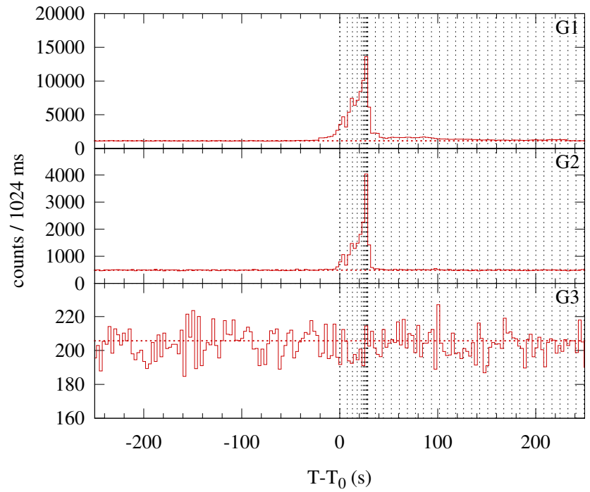
Konus-WIND S1 SOL1998-11-05T13:34 (M1.5) T_0 = 48882.668 s UT (13:34:42.668)
