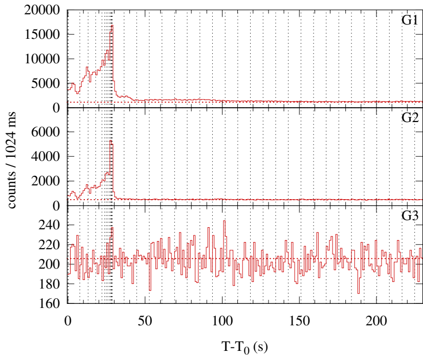
Konus-WIND S1 SOL1998-11-05T13:34 (M1.5) T_0 = 48882.668 s UT (13:34:42.668)
