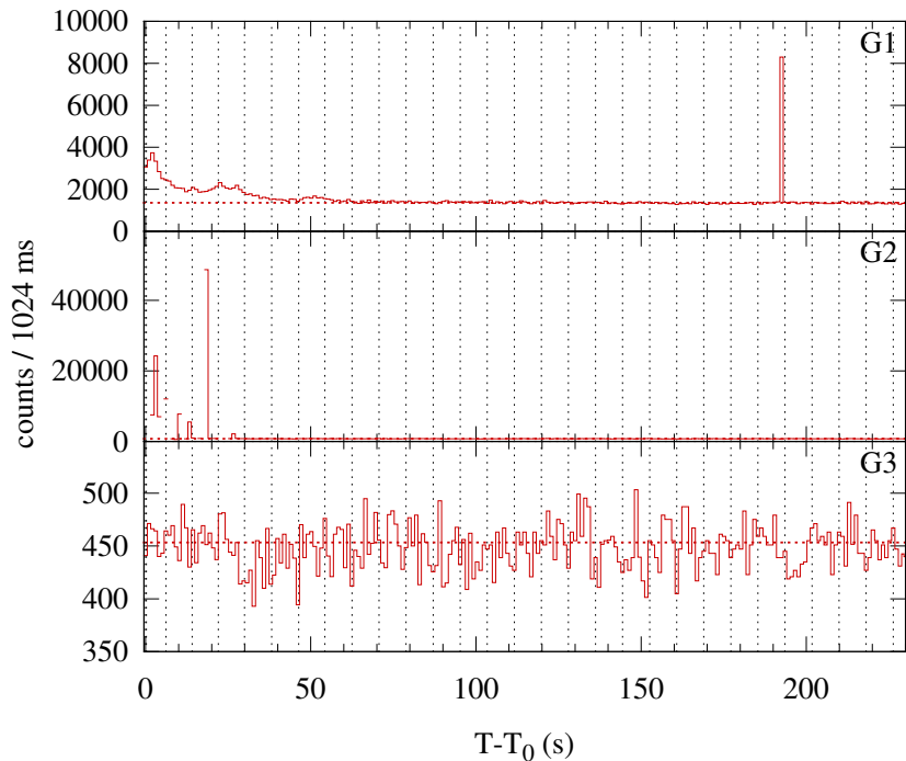
Konus-WIND S2 SOL1998-11-16T20:14 (C7.9) T 0 = 72882.5 s UT (20:14:42.5)
