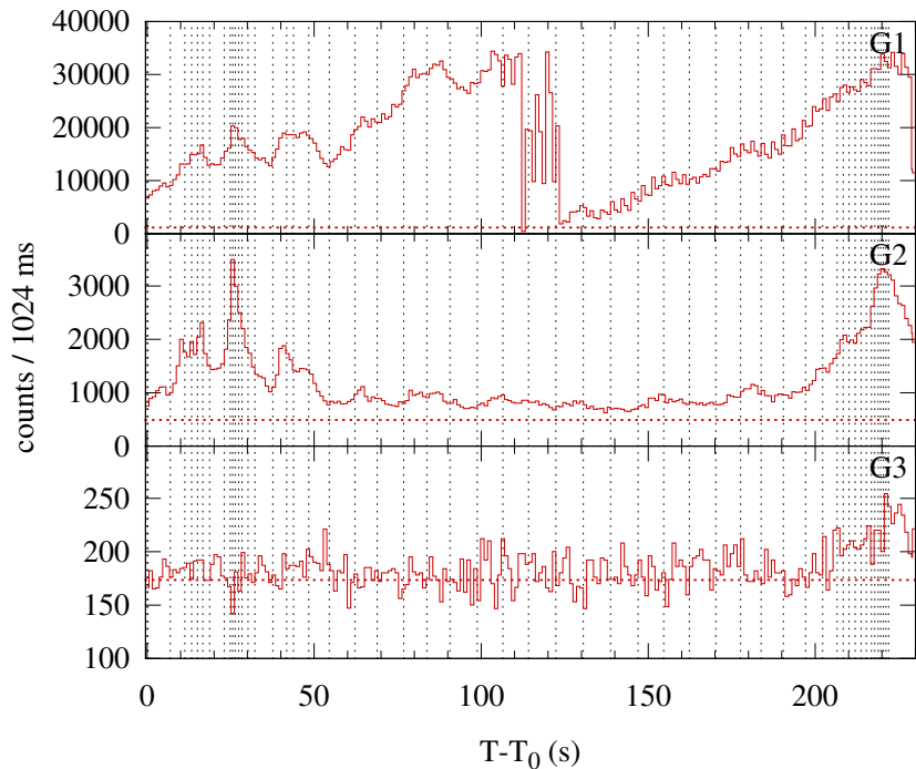
Konus-WIND S2 SOL1998-11-22T16:16 (X2.5) T_0 = 58619.364 s UT (16:16:59.364)
