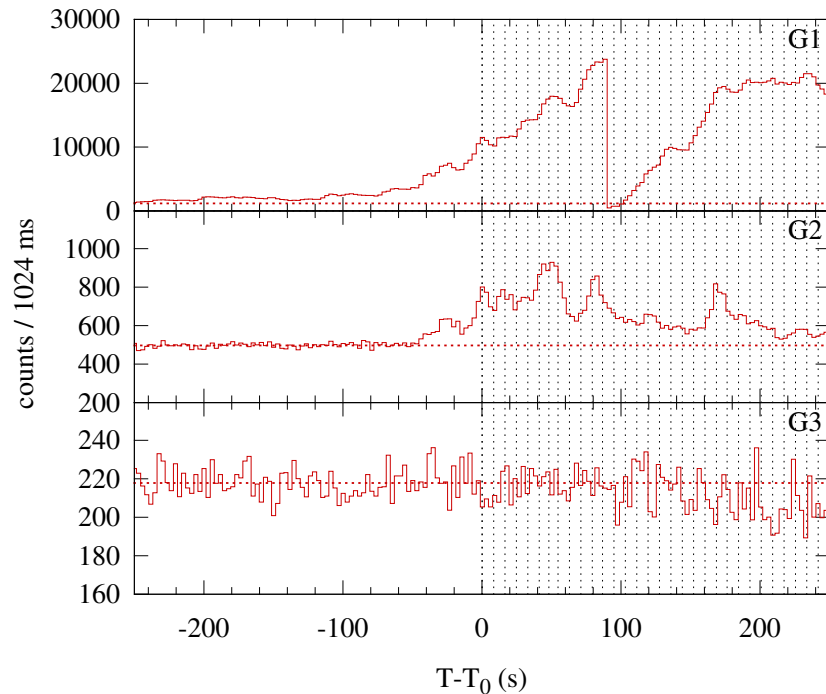
Konus-WIND S1 SOL1998-11-23T06:34 (X2.2) T_0 = 23672.275 s UT (06:34:32.275)
