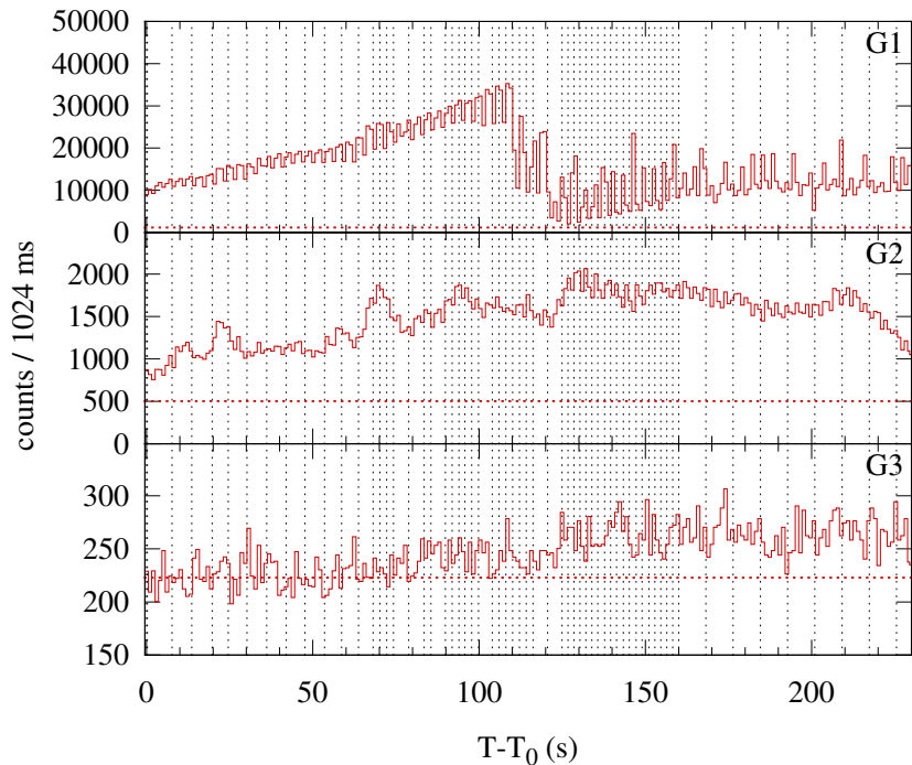
Konus-WIND S1 SOL1998-11-24T02:11 (X1.0) T_0 = 7891.959 s UT (02:11:31.959)
