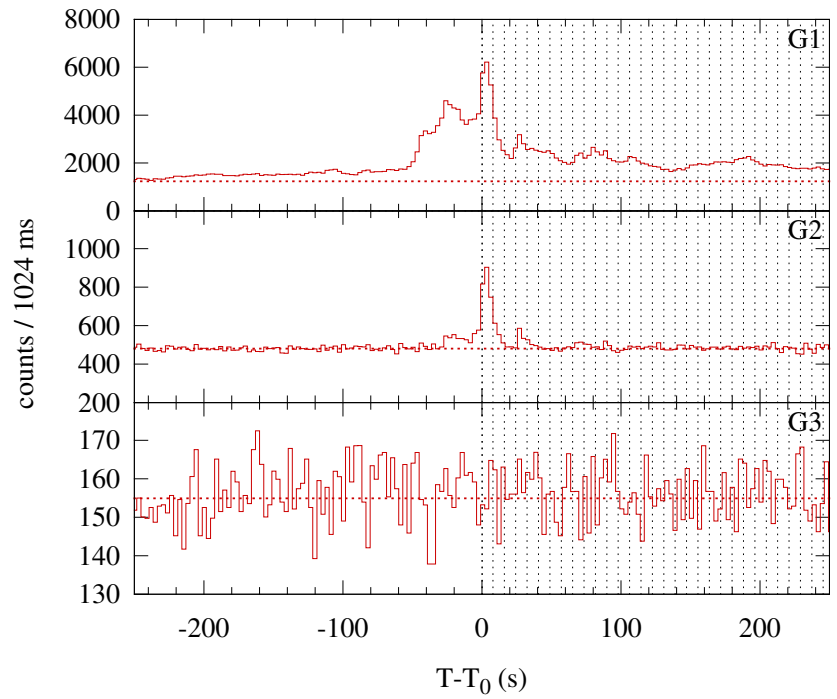
Konus-WIND S2 SOL1998-12-24T11:40 (M1.7) T_0 = 42040.661 s UT (11:40:40.661)
