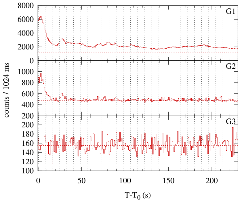
Konus-WIND S2 SOL1998-12-24T11:40 (M1.7) T_0 = 42040.661 s UT (11:40:40.661)
