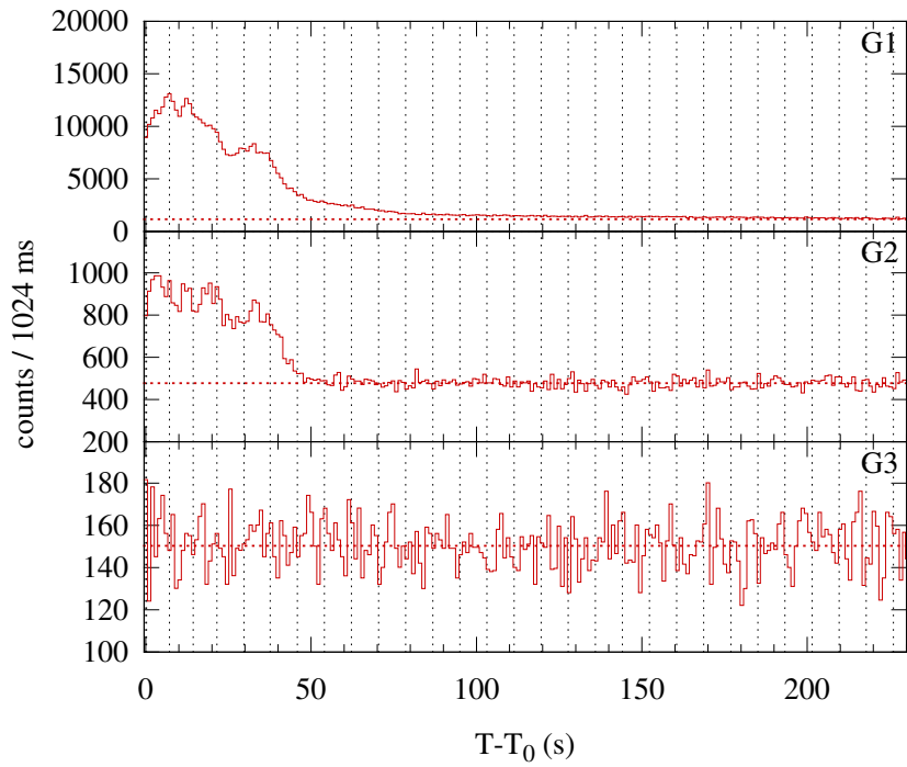
Konus-WIND S2 SOL1998-12-28T05:46 (M3.1) T_0 = 20797.759 s UT (05:46:37.759)
