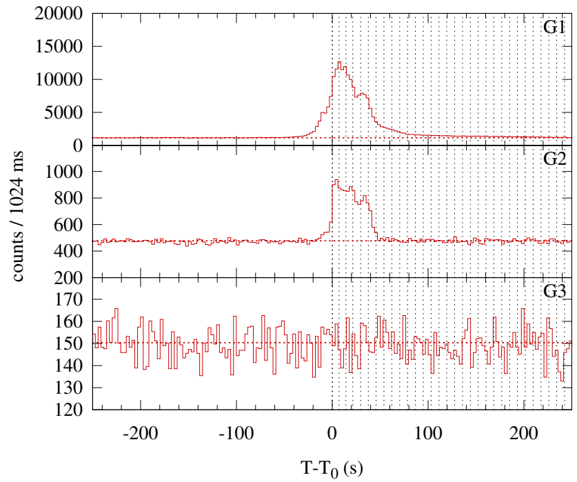
Konus-WIND S2 SOL1998-12-28T05:46 (M3.1) T_0 = 20797.759 s UT (05:46:37.759)
