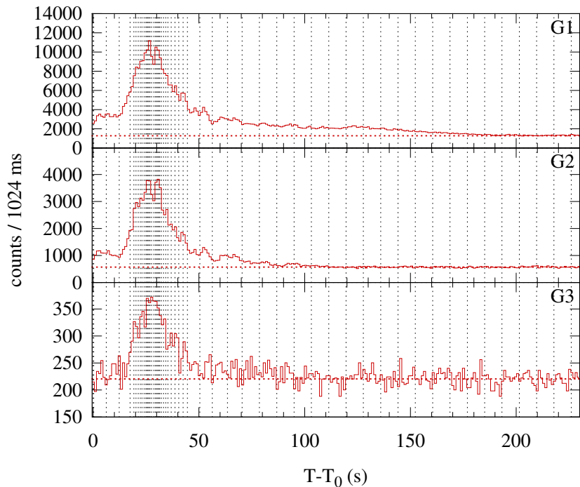
Konus-WIND S2 SOL1999-01-25T00:54 (M2.6) T_0 = 3275.723 s UT (00:54:35.723)
