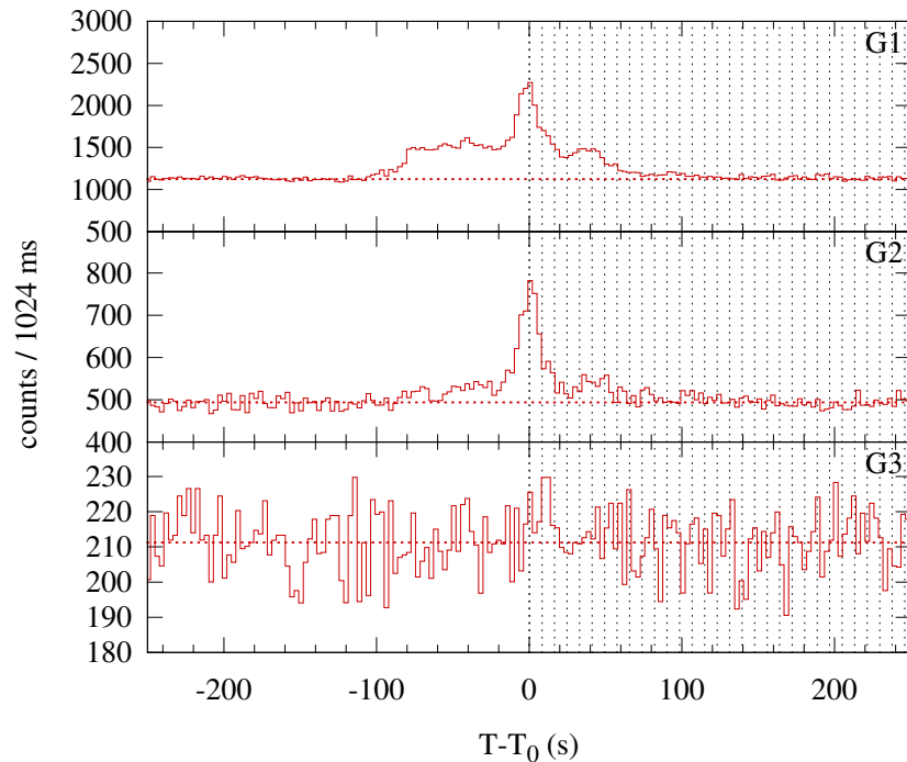
Konus-WIND S1 SOL1999-01-26T18:41 (C7.9) T 0 = 67270.478 s UT (18:41:10.478)
