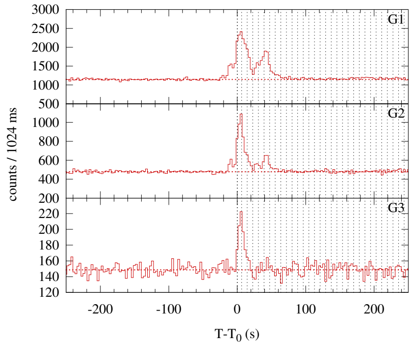
Konus-WIND S2 SOL1999-02-01T08:36 (C3.8) T 0 = 30992.532 s UT (08:36:32.532)
