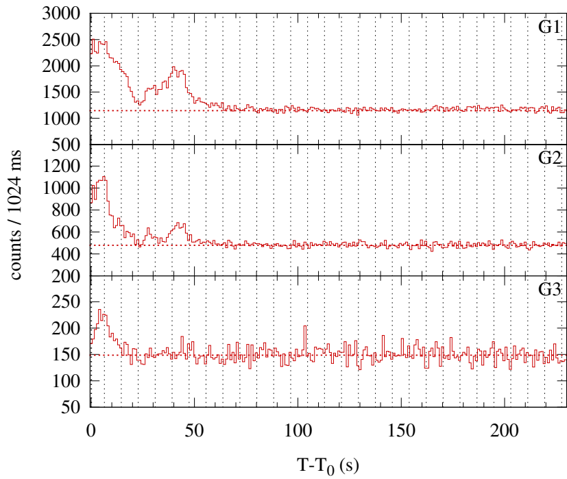
Konus-WIND S2 SOL1999-02-01T08:36 (C3.8) T 0 = 30992.532 s UT (08:36:32.532)
