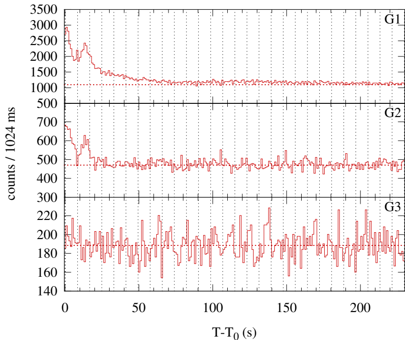
Konus-WIND S1 SOL1999-02-13T16:10 (C9.4) T 0 = 58259.920 s UT (16:10:59.920)
