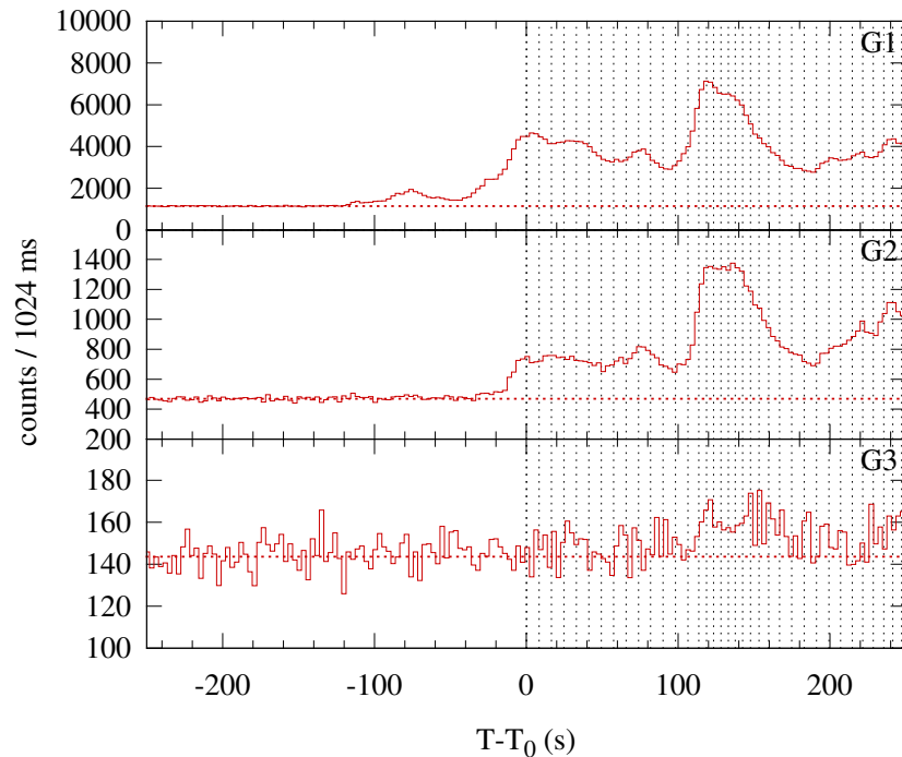
Konus-WIND S2 SOL1999-02-16T02:54 (M3.2) T_0 = 10447.985 s UT (02:54:07.985)
