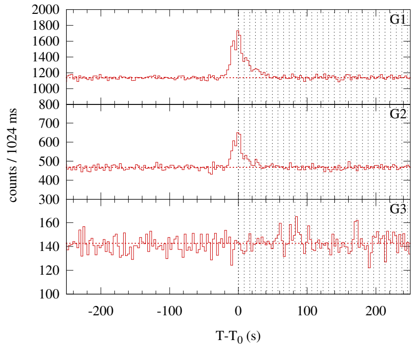
Konus-WIND S2 SOL1999-02-17T16:30 (C3.4) T_0 = 59420.507 s UT (16:30:20.507)
