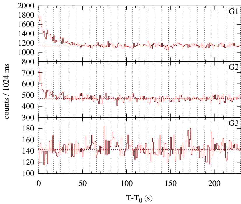
Konus-WIND S2 SOL1999-02-17T16:30 (C3.4) T_0 = 59420.507 s UT (16:30:20.507)
