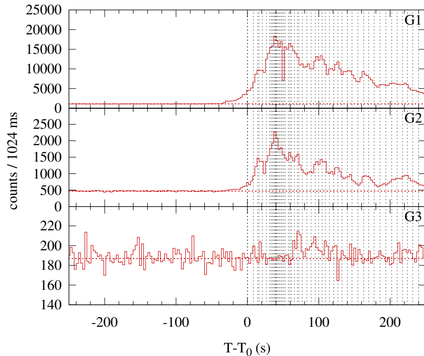
Konus-WIND S1 SOL1999-02-28T16:35 (M6.6) T 0 = 59732.55 s UT (16:35:32.55)
