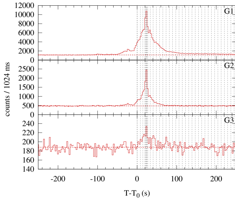
Konus-WIND S1 SOL1999-03-08T06:34 (M2.6) T_0 = 23693.829 s UT (06:34:53.829)
