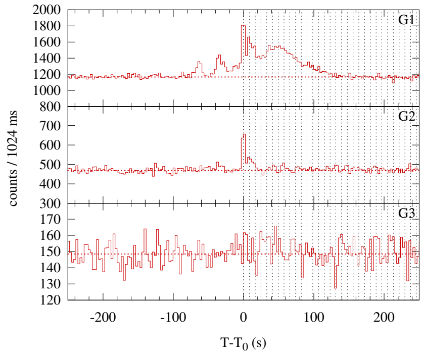
Konus-WIND S2 SOL1999-03-11T00:08 (C8.7) T 0 = 489.62 s UT (00:08:09.62)
