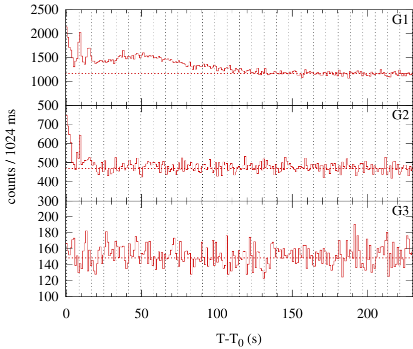
Konus-WIND S2 SOL1999-03-11T00:08 (C8.7) T 0 = 489.62 s UT (00:08:09.62)
