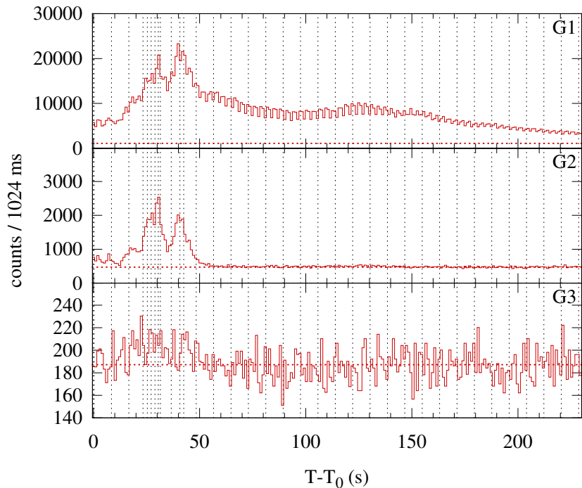
Konus-WIND S1 SOL1999-03-16T21:38 (M6.2) T 0 = 77895.88 s UT (21:38:15.88)
