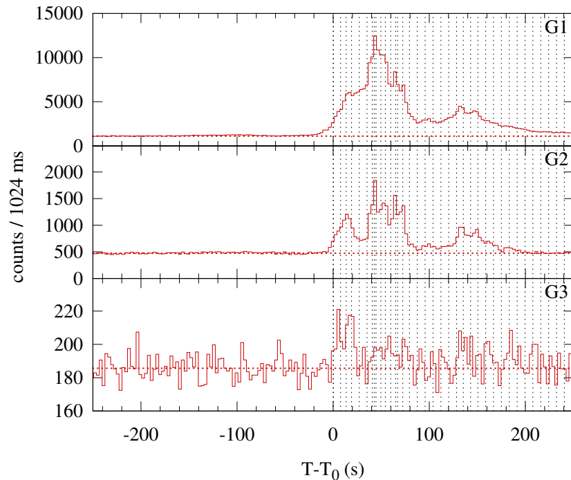
Konus-WIND S1 SOL1999-04-04T05:20 (M5.4) T 0 = 19244.502 s UT (05:20:44.502)
