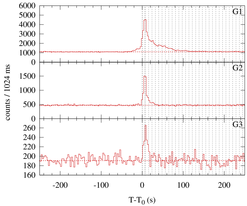
Konus-WIND S1 SOL1999-05-03T23:10 (M1.9) T_0 = 83413.180 s UT (23:10:13.180)
