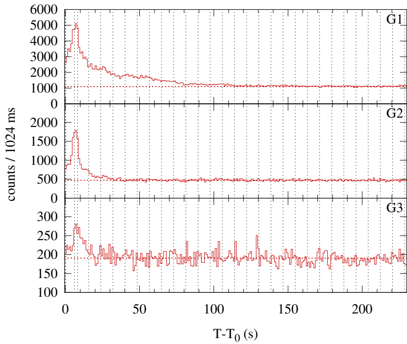
Konus-WIND S1 SOL1999-05-03T23:10 (M1.9) T_0 = 83413.180 s UT (23:10:13.180)
