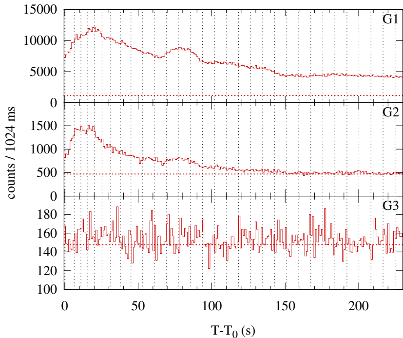
Konus-WIND S2 SOL1999-05-09T17:57 (M7.6) T 0 = 64651.918 s UT (17:57:31.918)
