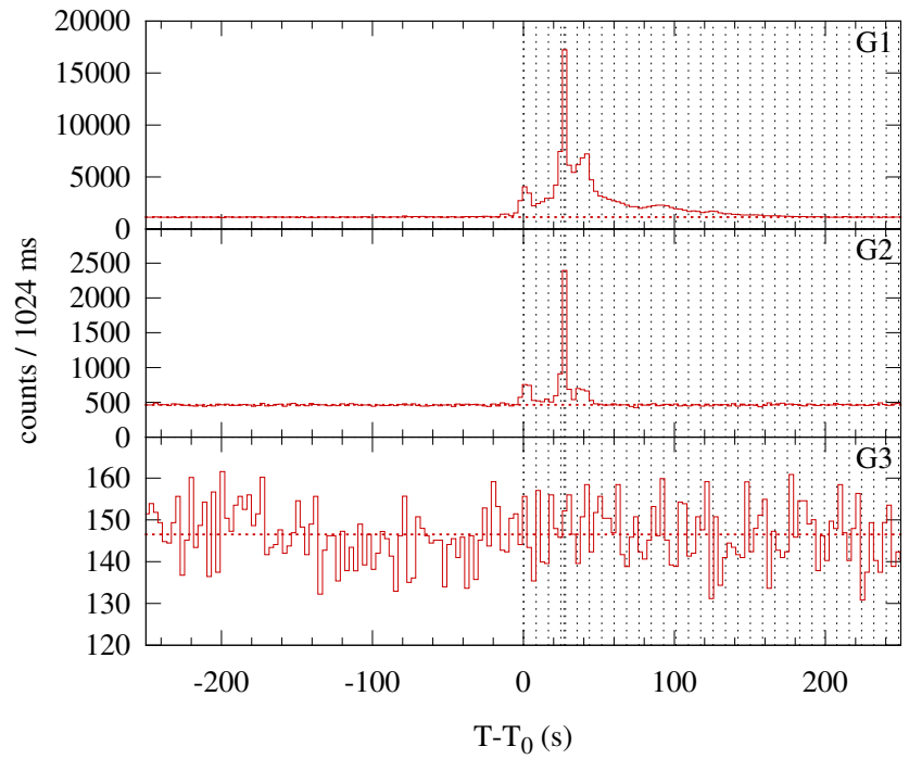
Konus-WIND S2 SOL1999-06-26T05:11 (M2.3) T 0 = 18670.257 s UT (05:11:10.257)
