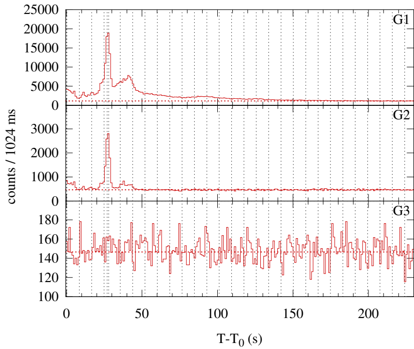
Konus-WIND S2 SOL1999-06-26T05:11 (M2.3) T 0 = 18670.257 s UT (05:11:10.257)
