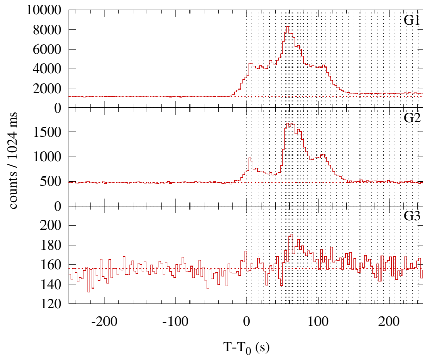
Konus-WIND S2 SOL1999-06-30T11:25 (M1.9) T 0 = 41137.211 s UT (11:25:37.211)
