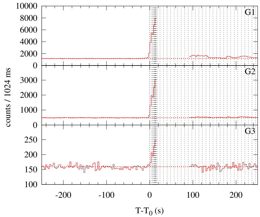
Konus-WIND S2 SOL1999-06-30T20:10 (M1.1) T_0 = 72605.479 s UT (20:10:05.479)
