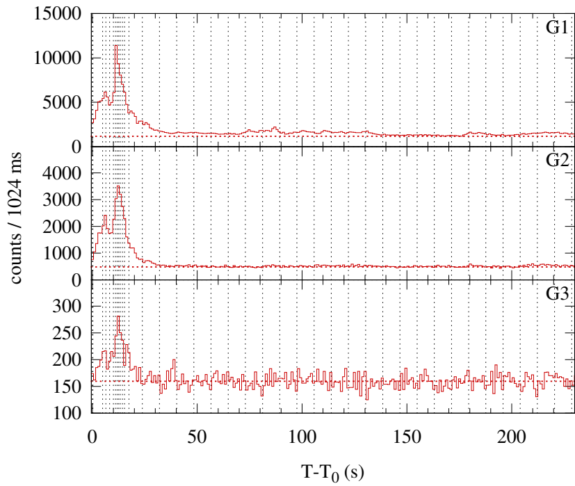
Konus-WIND S2 SOL1999-06-30T20:10 (M1.1) T_0 = 72605.479 s UT (20:10:05.479)
