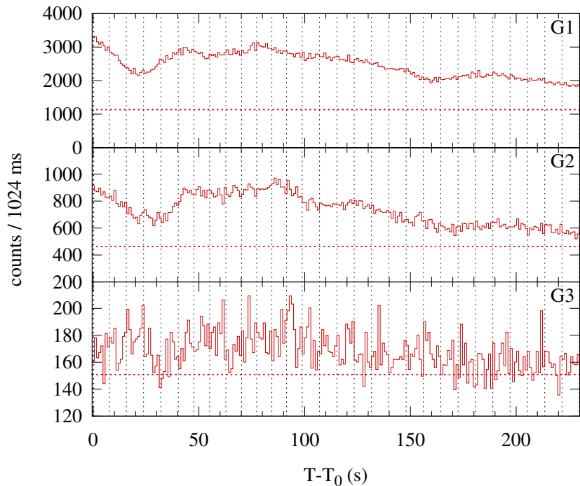
Konus-WIND S2 SOL1999-07-25T13:13 (M2.4) T 0 = 47608.201 s UT (13:13:28.201)
