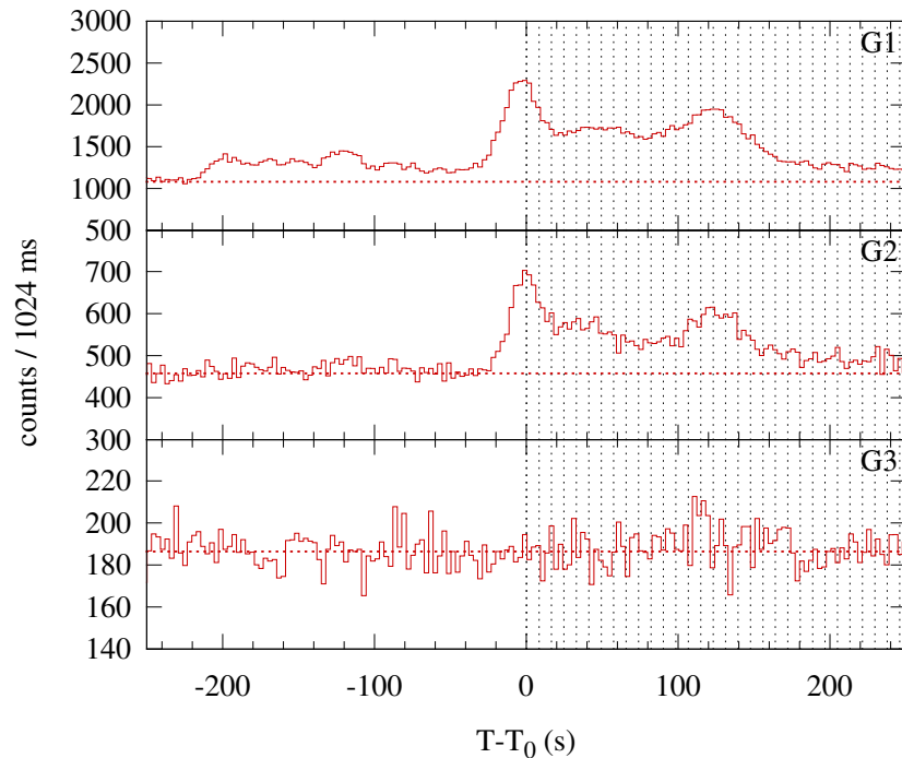
Konus-WIND S1 SOL1999-07-28T01:55 (M1.1) T 0 = 6910.860 s UT (01:55:10.860)
