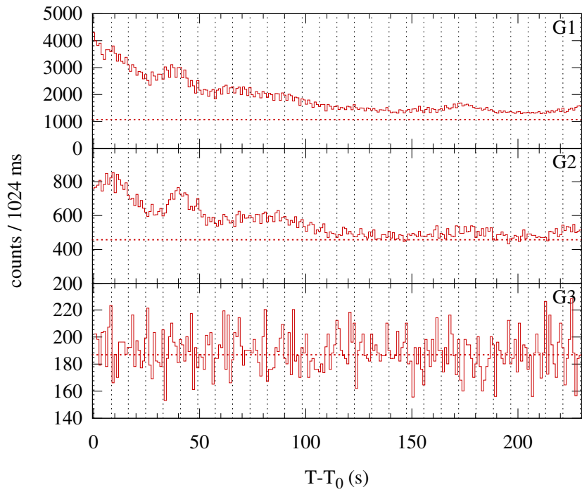
Konus-WIND S1 SOL1999-07-28T08:12 (M2.3) T_0 = 29558.586 s UT (08:12:38.586)
