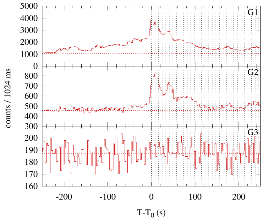
Konus-WIND S1 SOL1999-07-28T08:12 (M2.3) T_0 = 29558.586 s UT (08:12:38.586)
