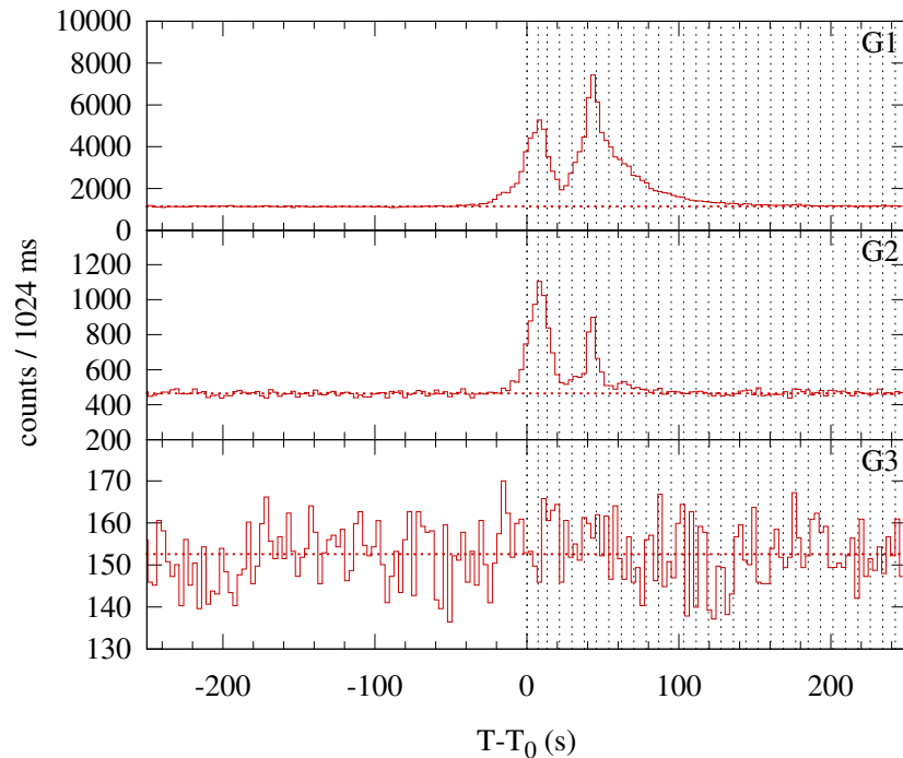
Konus-WIND S2 SOL1999-08-02T00:26 (M1.8) T 0 = 1560.81 s UT (00:26:00.81)
