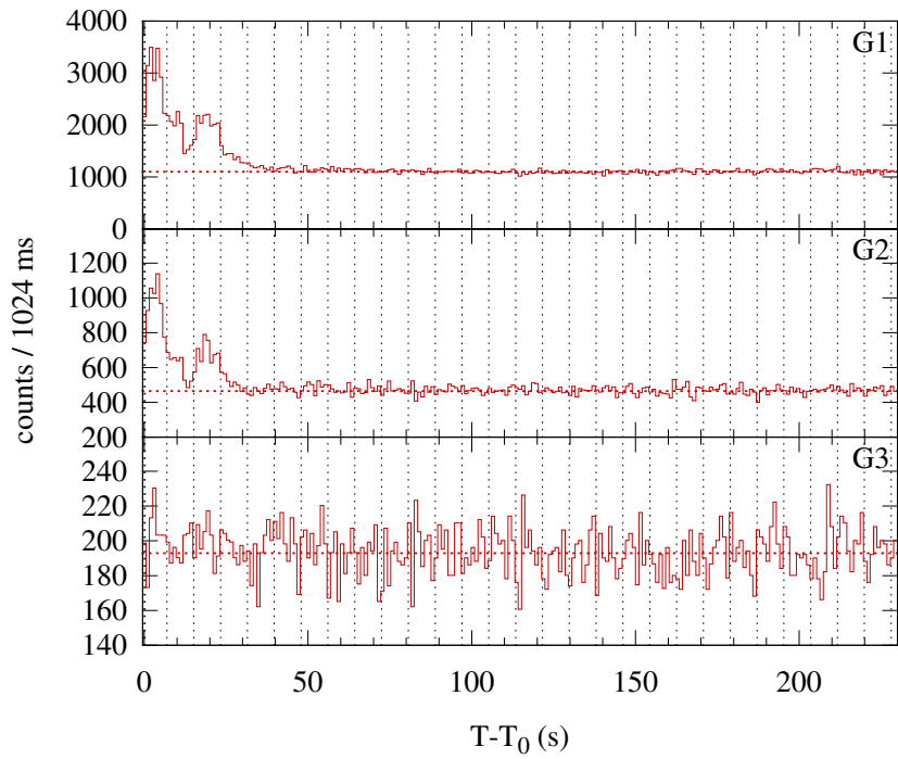
Konus-WIND S1 SOL1999-08-02T06:27 (C3.3) T_0 = 23257.501 s UT (06:27:37.501)
