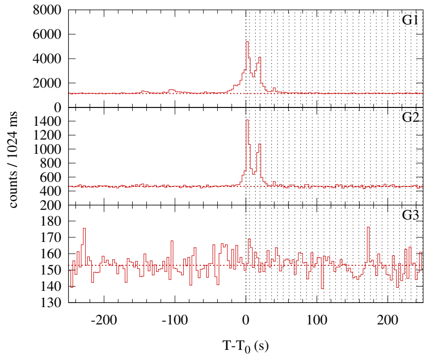
Konus-WIND S2 SOL1999-08-02T11:51 (C6.3) T 0 = 42703.651 s UT (11:51:43.651)
