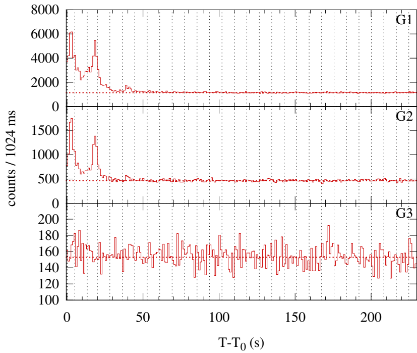
Konus-WIND S2 SOL1999-08-02T11:51 (C6.3) T 0 = 42703.651 s UT (11:51:43.651)
