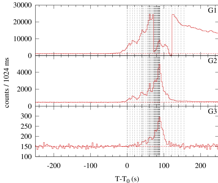
Konus-WIND S2 SOL1999-08-02T21:21 (X1.4) T_0 = 76909.107 s UT (21:21:49.107)
