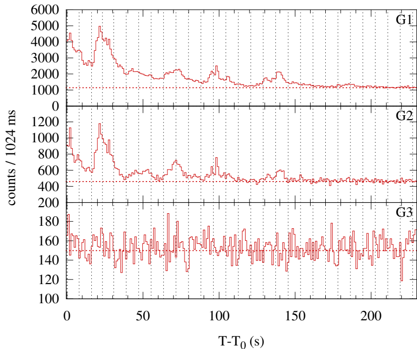
Konus-WIND S2 SOL1999-08-14T12:06 (C7.2) T_0 = 43609.161 s UT (12:06:49.161)
